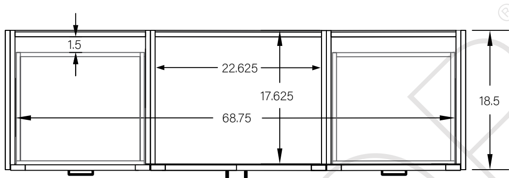
TOP VIEW
