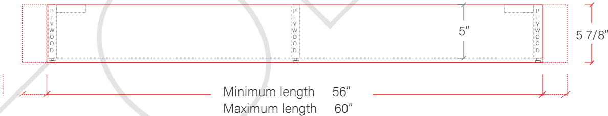
FRONT VIEW
