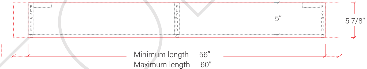
FRONT VIEW
