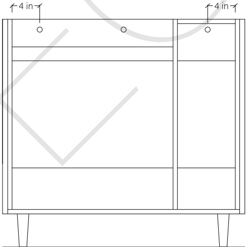
INSIDE BACK VIEW
